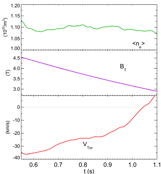
FIG. 11. Time histories of the electron density (top), toroidal magnetic field (middle), and core rotation velocity (bottom) in a 0.8 MA plasma with a downward magnetic field ramp.
